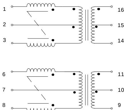
SCHEMATIC
