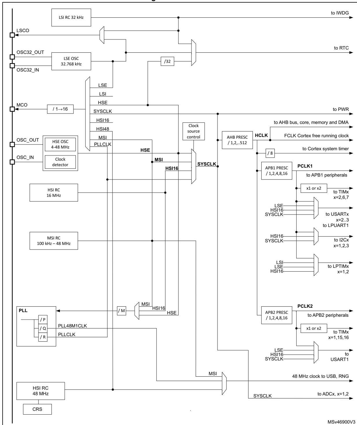
Figure 5. Clock tree
