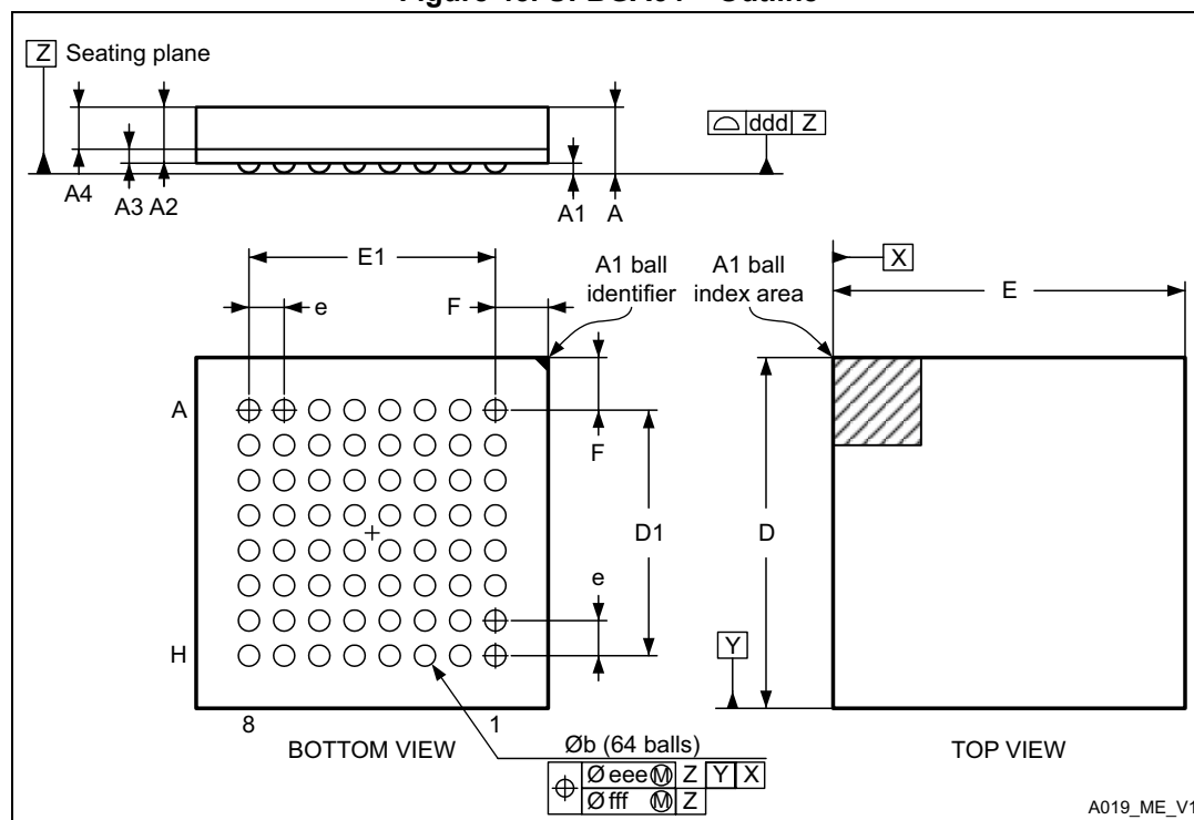
Figure 45. UFBGA64 – Outline
