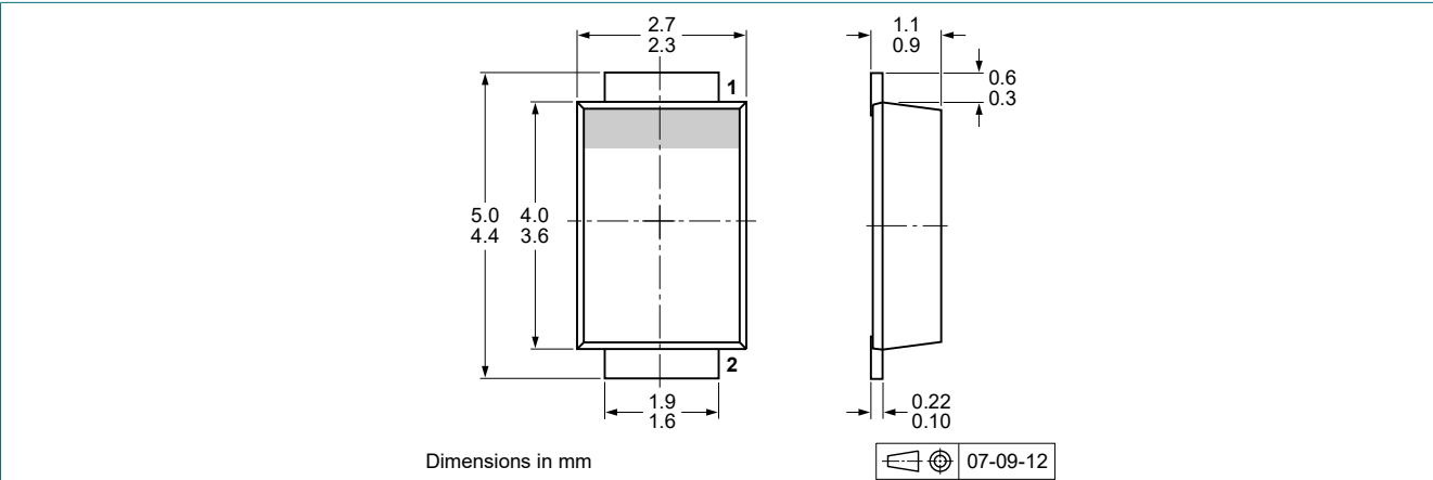
Fig. 16. Package outline CFP5 (SOD128)
