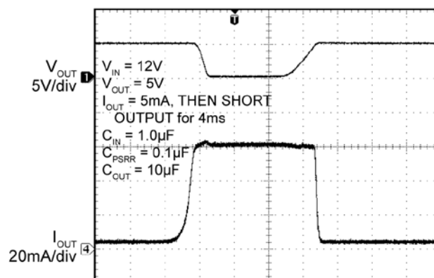
Current Limit
