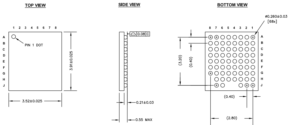
Figure 9. 68-Ball WLCSP Package Outline
