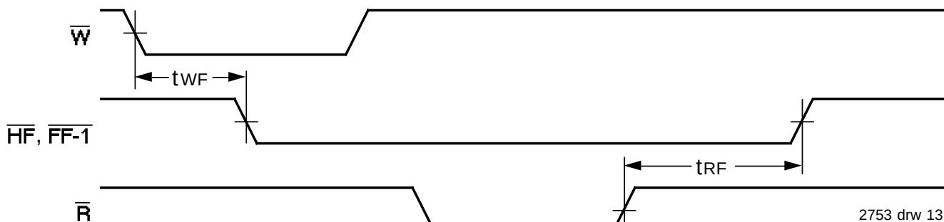
Figure 10. Half-Full and Full-minus-1 Flag Timings
