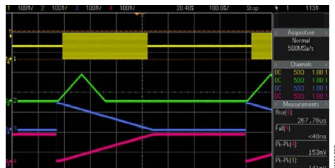
Figure 58. Programming Example 4
