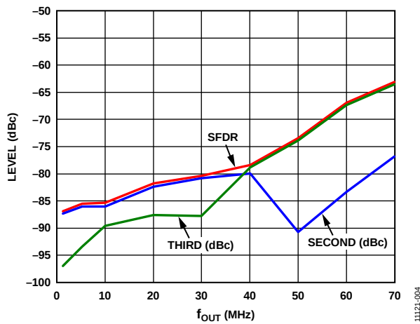
Figure 4. SFDR, Second and Third Harmonics vs. f_{OUT} , I_{OUTS} = 4 mA
