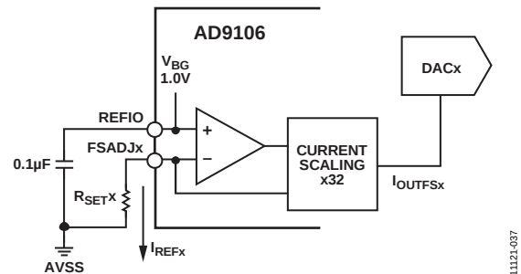
Figure 36. On-Chip Reference with External xR_{SET} Resistor
