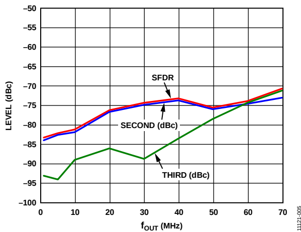
Figure 5. SFDR, Second and Third Harmonics vs. f_{OUT} , I_{OUTS} = 2 mA
