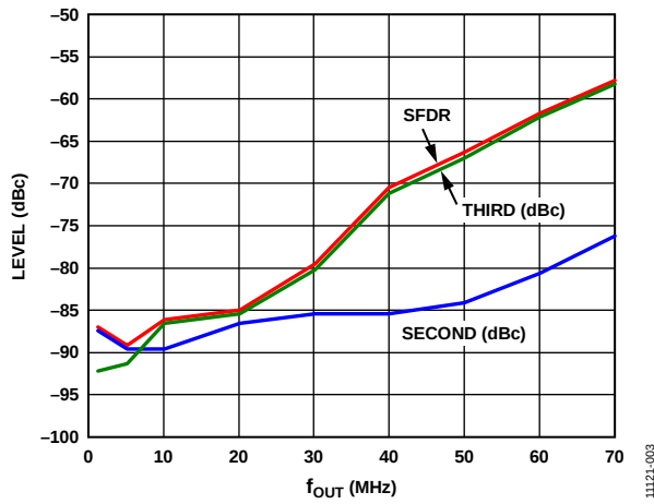
Figure 3. SFDR, Second and Third Harmonics vs. f_{OUT} , I_{OUTS} = 8 mA
