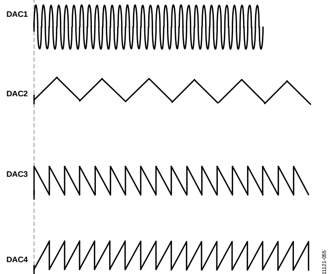
Figure 54. Waveforms Without Start Delays
