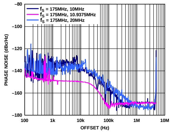
Figure 17. Phase Noise
