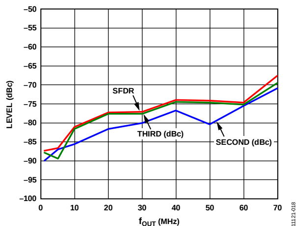
Figure 18. SFDR, Second and Third Harmonics vs. f_{OUT} , I_{OUTS} = 4 mA
