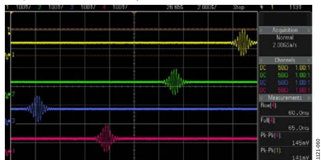
Figure 59. Programming Example 5
