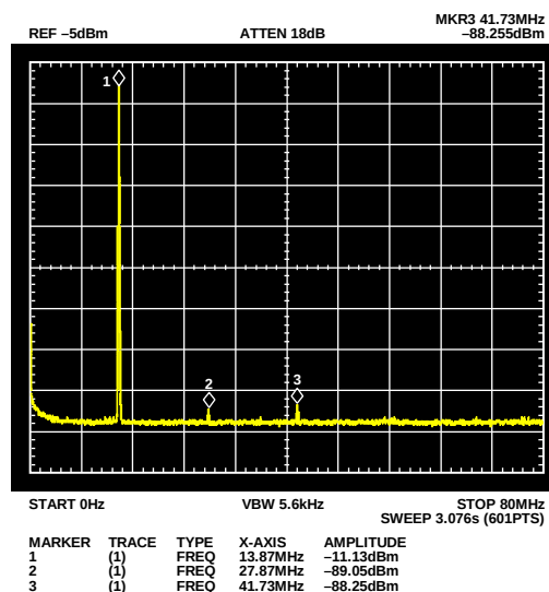
Figure 23. Output Spectrum, f_{OUT} = 13.87 MHz
