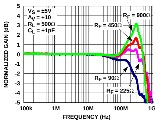
FIGURE 12. GAIN vs FREQUENCY FOR VARIOUS R_F ( A_V = +10 )
