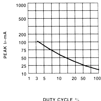
Fig. 6 MAX PEAK CURRENT VS. DUTY CYCLE % (REFRESH f = 1 \text{ KHz} )
