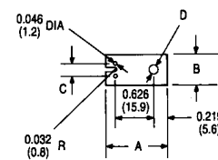
TO-66 (RECTANGLE)
