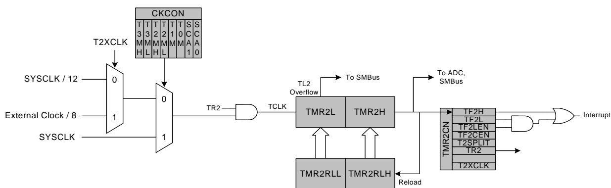
Figure 28.4. Timer 2 16-Bit Mode Block Diagram
