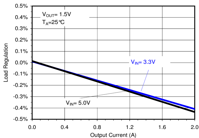
Load Regulation ( V_{OUT}=1.5V )
