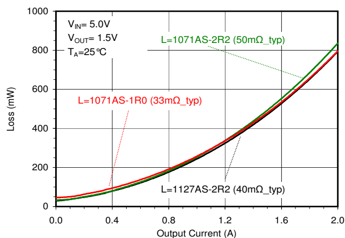
Total Loss vs. Load Current ( V_{OUT}=1.5V )
