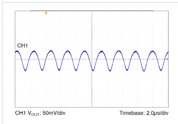
Figure 40 — Output Ripple: 48V IN , 12.0V OUT at 9A. V_{OUT} = 50\text{mV}/\text{Div} , 2.0μs/Div; C_{OUT} = 6 \times 10\mu\text{F} Ceramic
