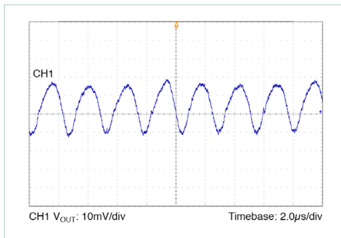
Figure 42 — Output Ripple: 48V IN , 12.0V OUT at 4.5A. V_{OUT} = 10\text{mV}/\text{Div} , 2.0μs/Div; C_{OUT} = 6 \times 10\mu\text{F} Ceramic
