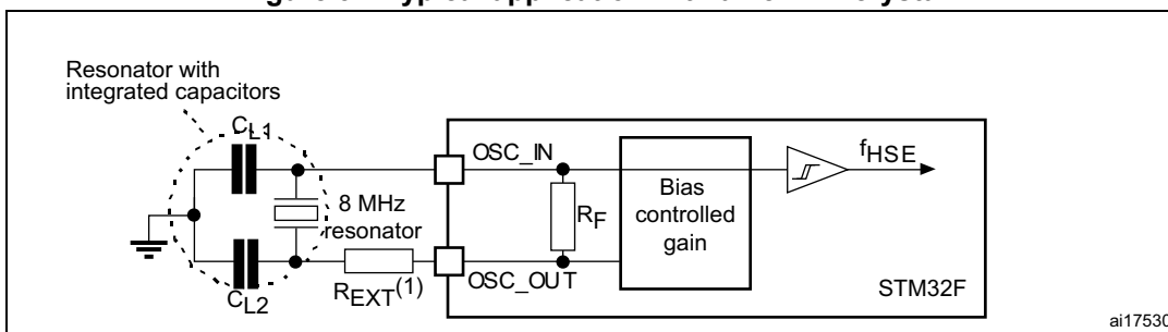
Figure 31. Typical application with an 8 MHz crystal
