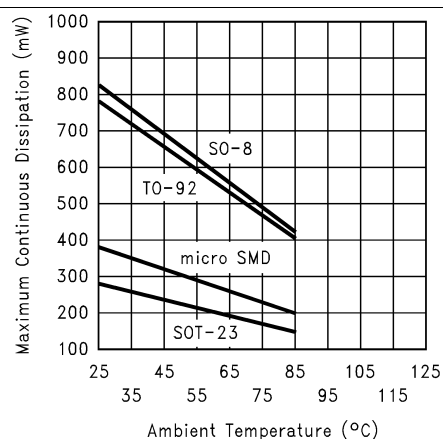
Figure 14. Thermal Information
