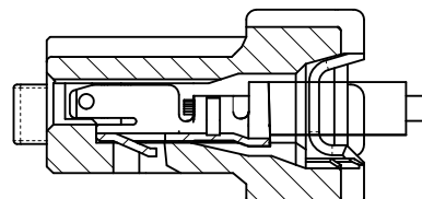
MATED CONDITION (REFERENCE)
