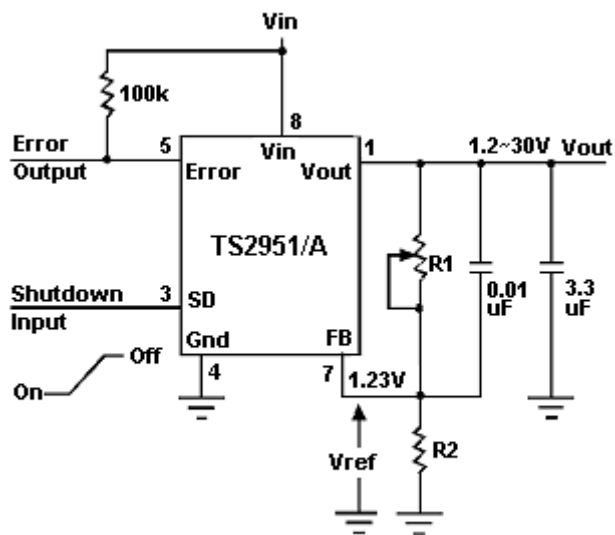
Figure 2. Adjust Voltage
