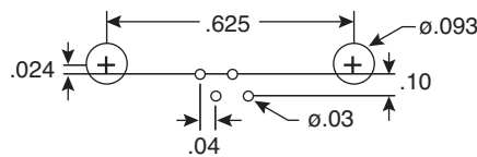
PCB Layout (4 Contact)
