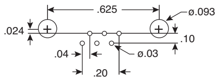
PCB Layout (6 Contact)
