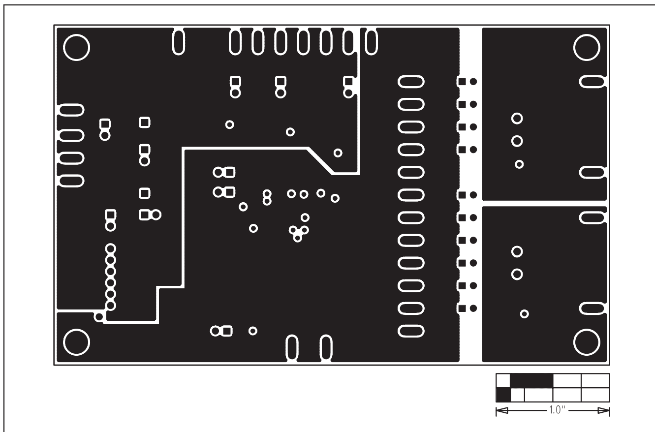
Figure 10. MAX11008 EV Kit PCB Layout—Ground Layer 2
