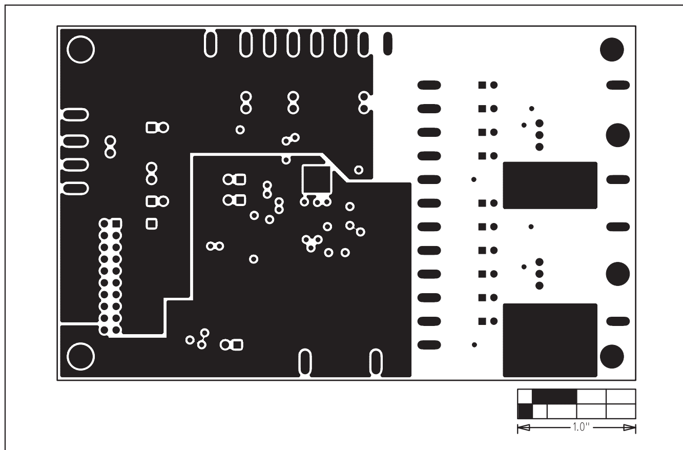
Figure 11. MAX11008 EV Kit PCB Layout—Power Layer 3
