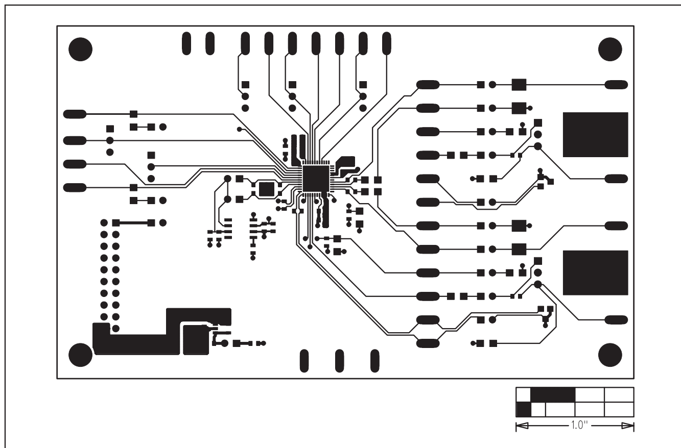
Figure 9. MAX11008 EV Kit PCB Layout—Component Side
