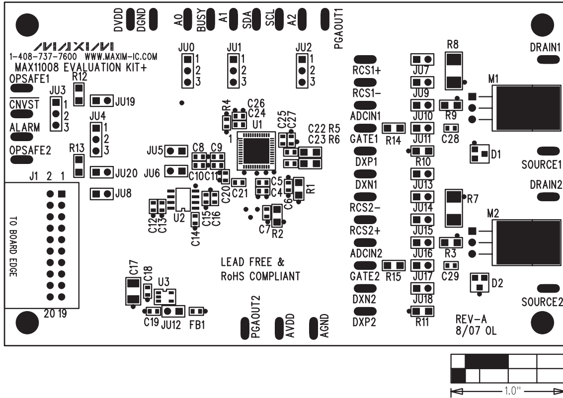
Figure 8. MAX11008 EV Kit Component Placement Guide—Component Side
