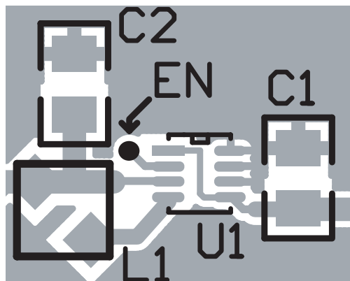
Figure 2: Component Placement.
