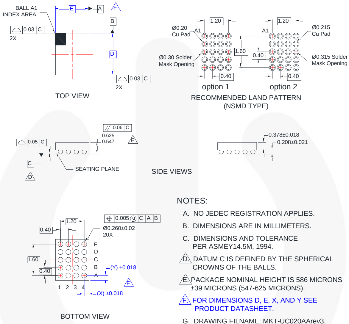
Figure 41. 20-Ball, Wafer-Level Chip-Scale Package (WLCSP), 4x5 Array, 0.4 mm Pitch, 250 \mu m Ball
