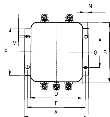
Housing L1
