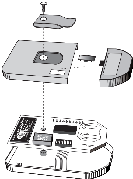
Figure 9: CMD-HHCP-***-MD Assembly
