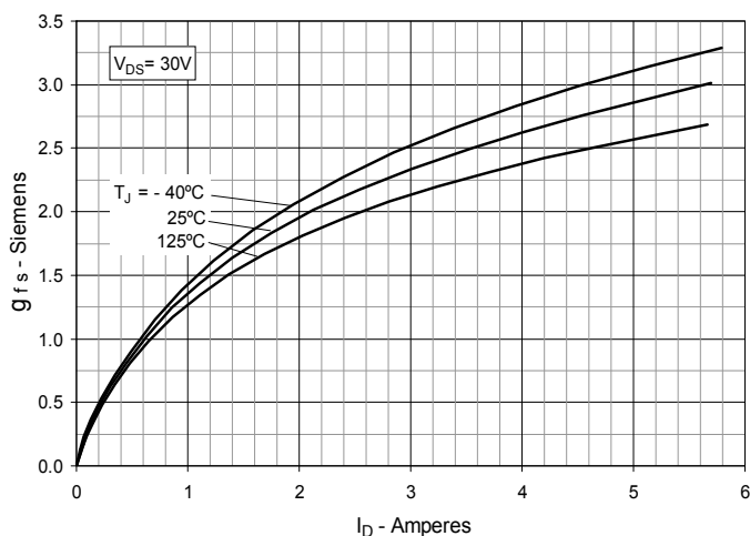
Fig. 10. Transconductance
