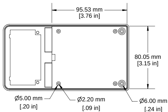
BOX - INSIDE
