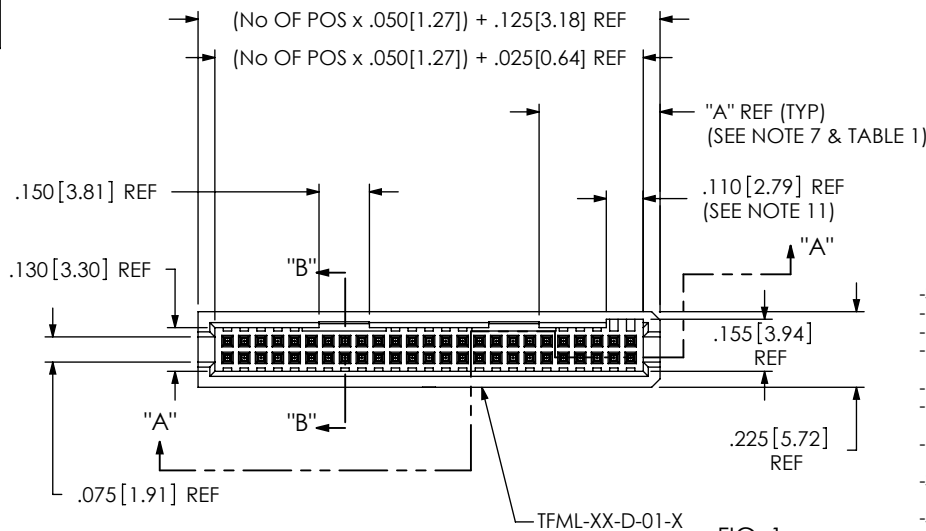
FIG. 1 -01: THROUGH HOLE
