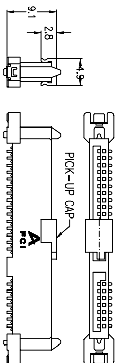
PART WITH PICK-UP CAP (XXXXXX-XXXXCLF)
