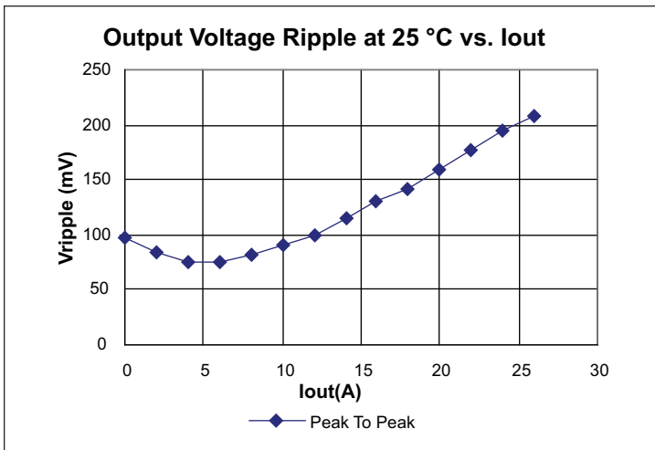
Figure 7 — Ripple vs. I_{OUT} ; 352 V_{IN} , no external capacitance
