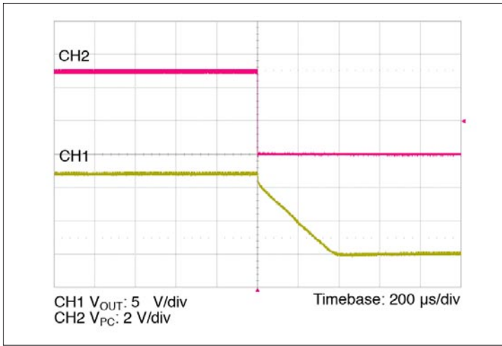
Figure 13 — PC disable waveform, 352 V_{IN} , 1000 \mu F C_{OUT} full load
