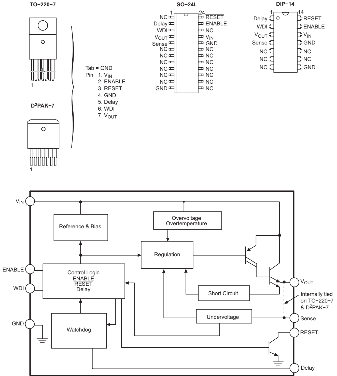
Figure 1. Block Diagram
