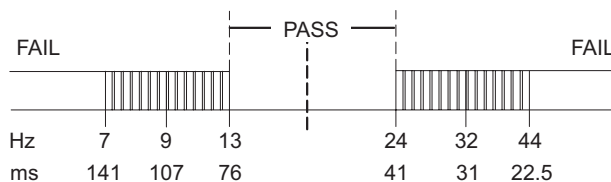
Figure 19. WDI Signal for C_{\text{Delay}} = 0.82 \mu\text{F} using CS8140
