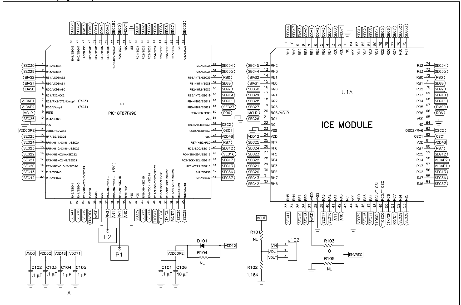
Board Schematic (Page 1 of 2)
