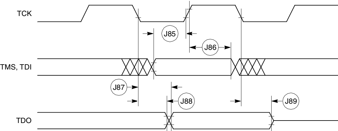
Figure 36. JTAG Test Access Port Timing Diagram
