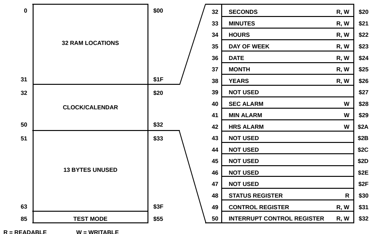
FIGURE 2. ADDRESS MAP
