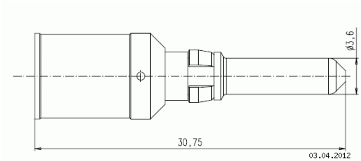
Drawing Dimensions in mm (Inch)
