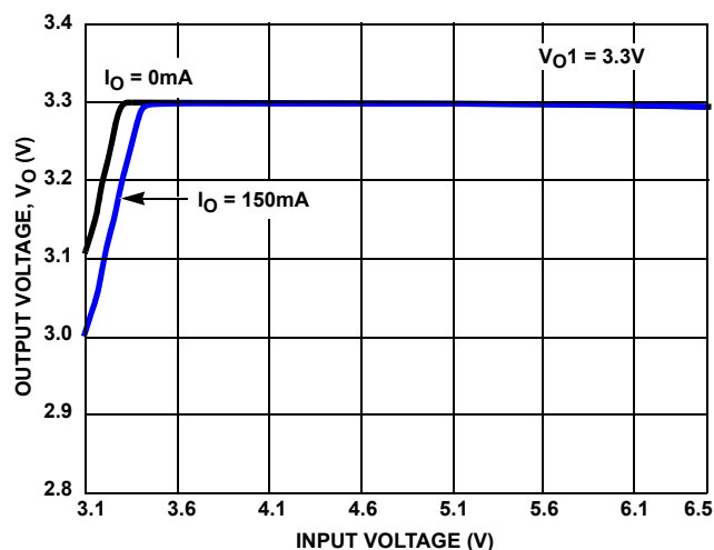
FIGURE 4. OUTPUT VOLTAGE vs INPUT VOLTAGE (V O1 = 3.3V)
