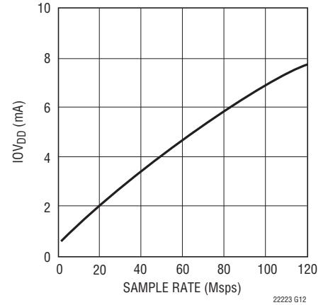
LTC2222: I_{OVD} vs Sample Rate, 5MHz Sine Wave Input, -1\text{dB} , 0V_{DD} = 1.8\text{V}
