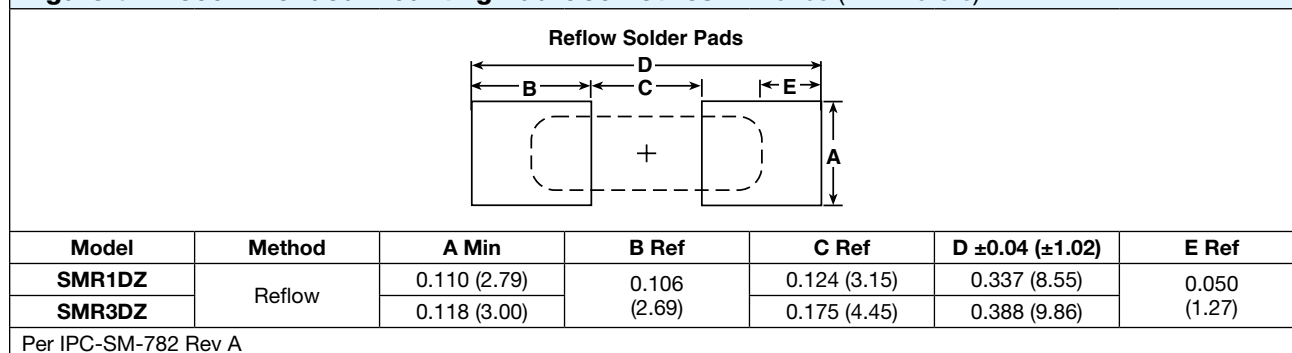
Figure 3—Recommended Mounting Pad Geometries in Inches (Millimeters)
