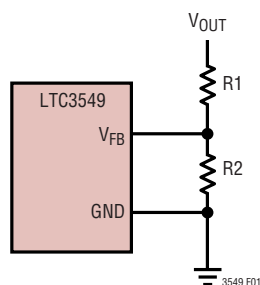
Figure 1. Setting the LTC3549 Output Voltage
