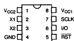
DS1302 8-PIN DIP (300 MIL)
