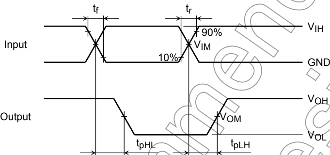
Figure 2 t_{pLH} , t_{pHL}
