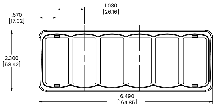
LM6 MOUNTING PANEL PANEL OPENING SIZE: 1.90 x 6.15 [48.3mm x 156.2mm]
