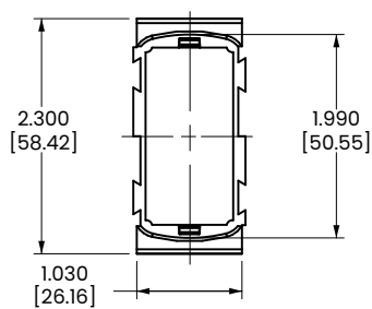
LMM MOUNTING PANEL MIDDLE
