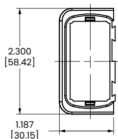
LME MOUNTING PANEL END
