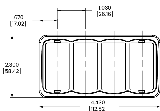
LM4 MOUNTING PANEL PANEL OPENING SIZE: 1.90 x 4.09 [48.3mm x 103.9mm]
