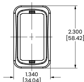
LMS MOUNTING PANEL
