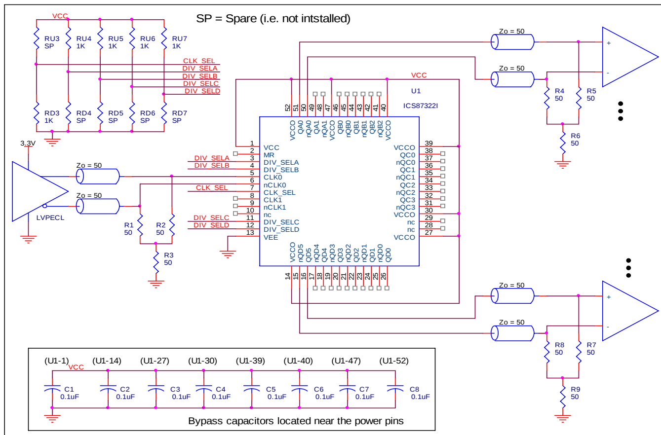
FIGURE 5. ICS87322BI SCHEMATIC EXAMPLE
