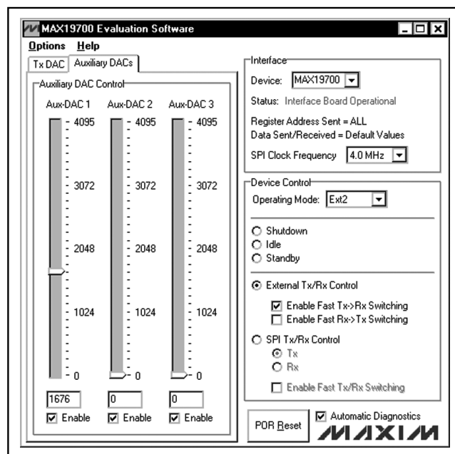
Figure 2. MAX19700 EV Kit Software Auxiliary DAC Control
