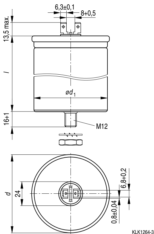
Dimensional drawing 2
