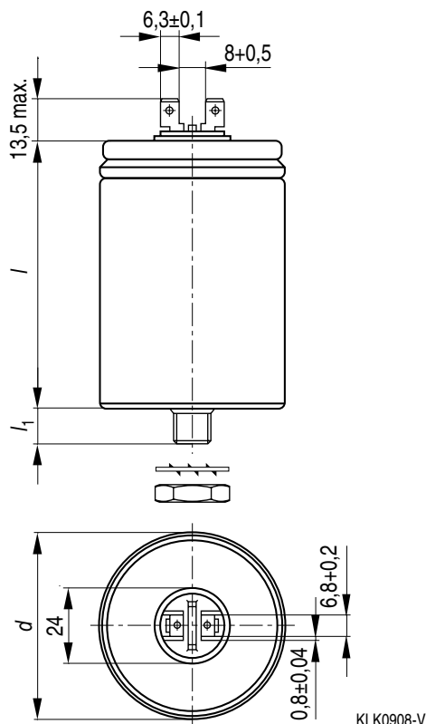
Dimensional drawing 1
