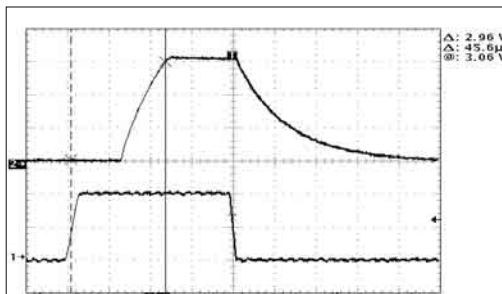
Turn-on Characteristic ( V_{IN} = 4V , I_{OUT}=100mA )
