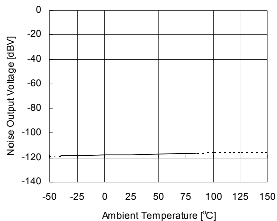
Noise Output Voltage vs. Ambient Temperature V+=9V, Rg=600Ω, A-Weighted
