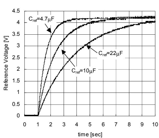
Reference Voltage Turn-on behaviour V_+=9V , T_a=25^{\circ}C
