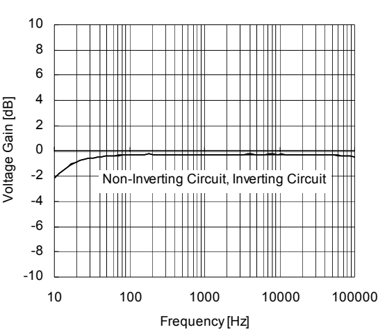
Voltage Gain vs. Frequency V_+=9V , V_{in}=1V_{rms} , T_a=25^{\circ}C
