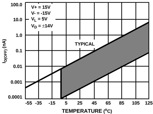
FIGURE 11. I_{D(OFF)} vs TEMPERATURE
