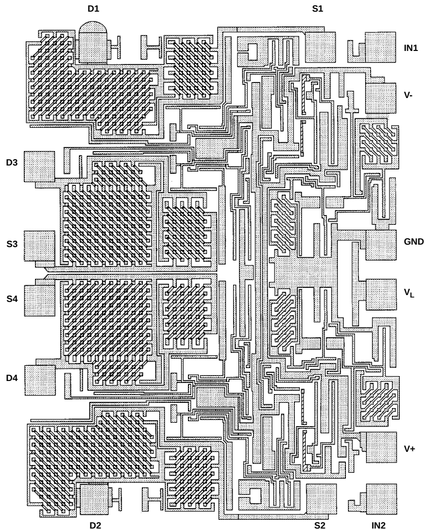
DG403/883, DG405/883
