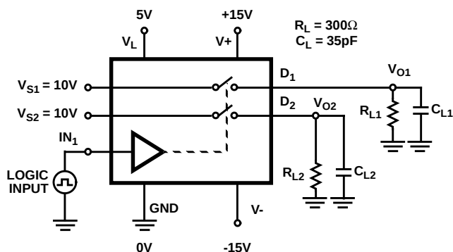
FIGURE 1. SWITCHING TIME
