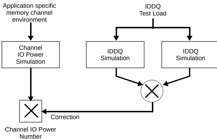
Figure 2 - Correlation from simulated Channel IO Power to actual Channel IO Power supported by I_{\text{DDQ}} Measurement
