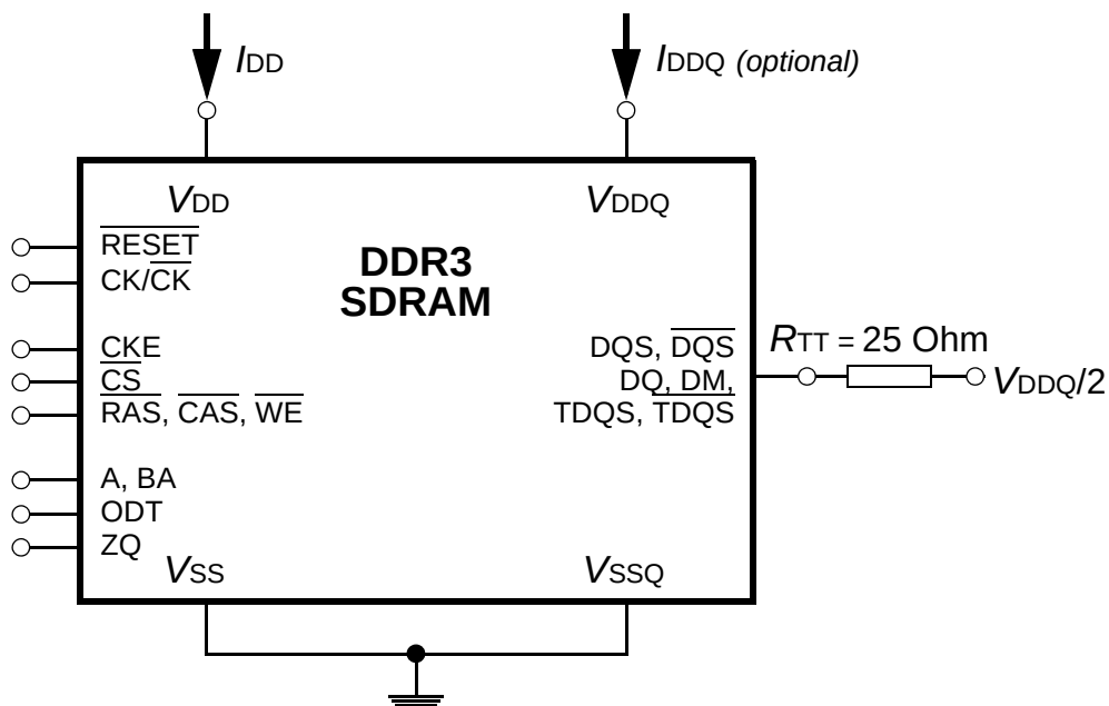
Figure 1 - Measurement Setup and Test Load for I_{\text{DD}} and I_{\text{DDQ}} (optional) Measurements [Note: DIMM level Output test load condition may be different from above]
