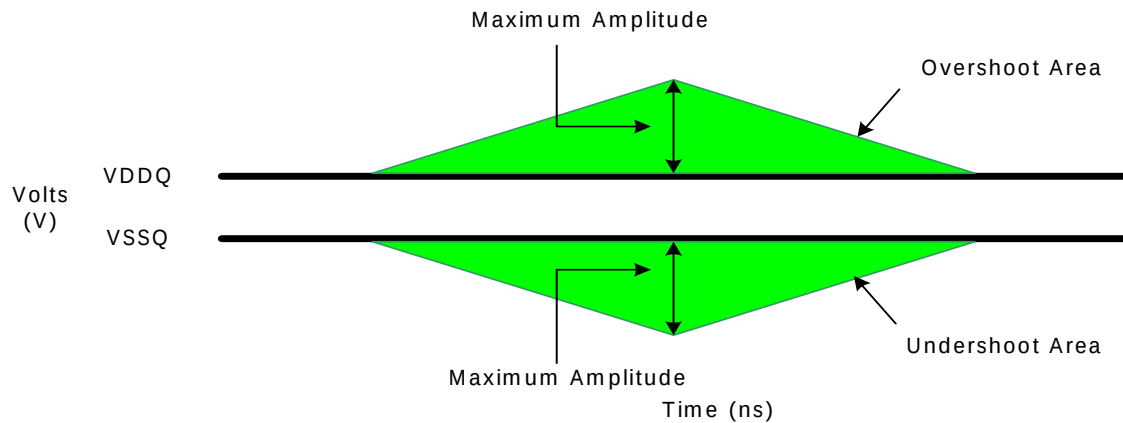
Clock, Data Strobe and Mask Overshoot and Undershoot Definition
