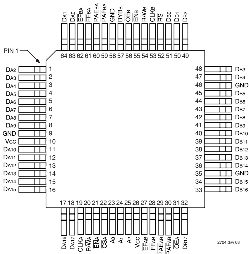
TQFP (PN64-1, order code: PF) TOP VIEW
