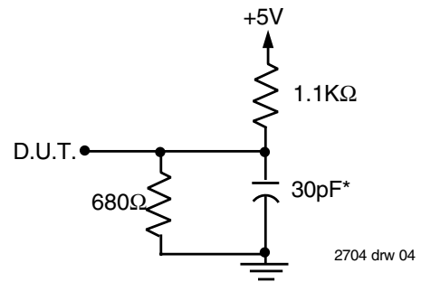
Figure 2. Output Load
