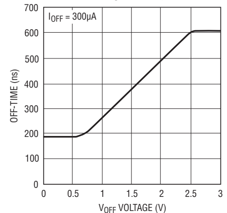
Off-Time vs V_{OFF} Voltage
