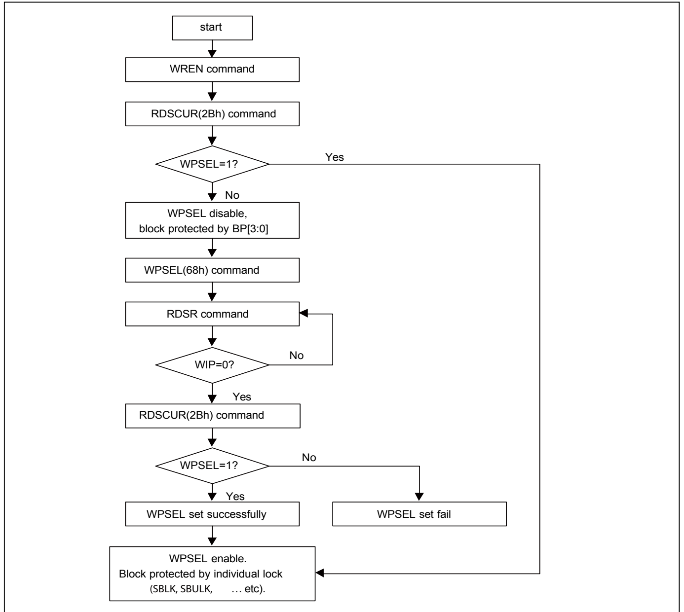
Figure 53. WPSEL Flow
